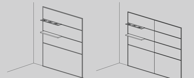
Telaio in alluminio H 225 a terra 4 elementi H 225 Aluminium frame up to the floor for 4 panels L. 150/200/300/400 - H. 225
